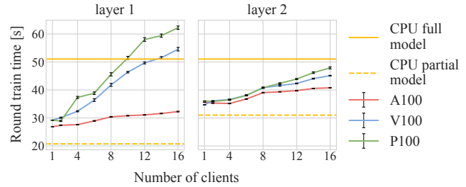
Figure 2: Round train time w.r.t. number of participating clients, size of the client model, and GPU type on the server.
